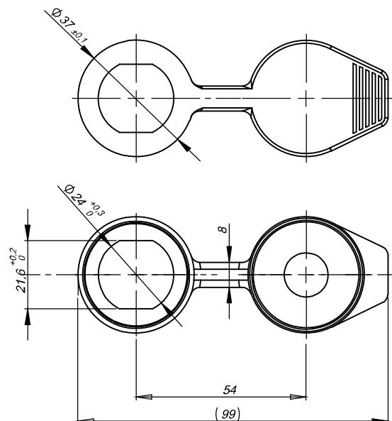
Cover 2.904.006
