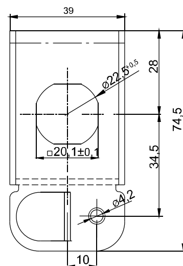
Blockade 2.905.002
