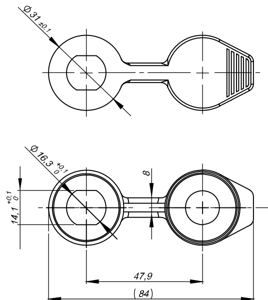
Cover 2.904.008
