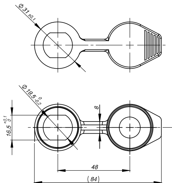
Cover 2.904.007
